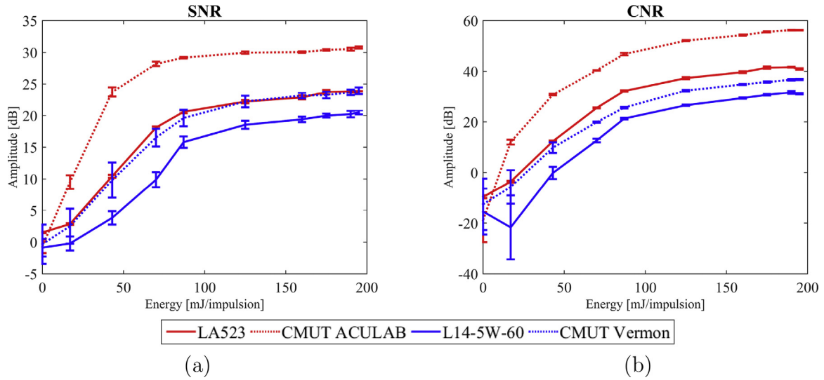
Fig. 9. Evolutions of the SNR and CNR as a function of the excitation energy for both probes types of each pair in the agar phantom (study 1 and 2, Table 2).
