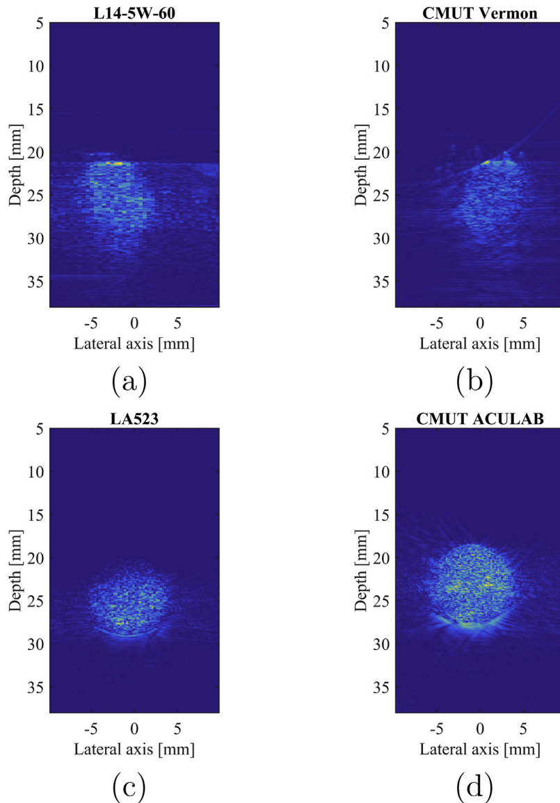
Fig. 8. PA images of the spherical inclusion made of coloured agar obtained with both probes of the two following pairs at 195 mJ/pulse: (a) L14-5W/60 (PZT) and (b) CMUT Vermon, and (c) LA523E (PZT) and (d) CMUT ACULAB.
